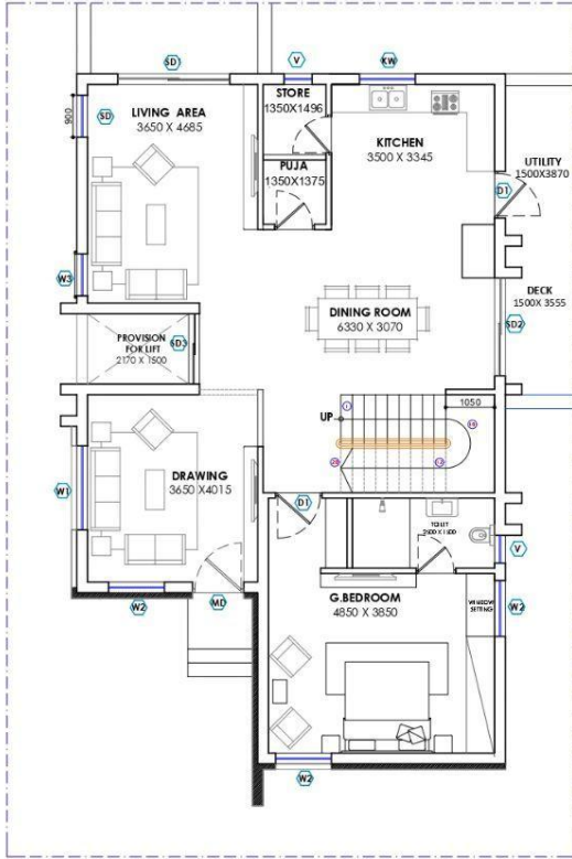
GROUND FLOOR PLAN V-31 (18-03-2023)
