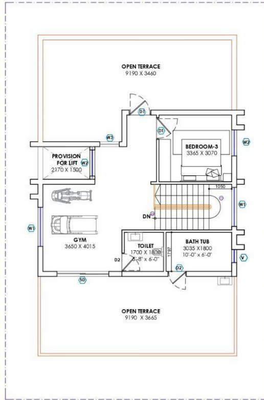
SECOND FLOOR PLAN- OP1 V-01 (18-03-2023)
