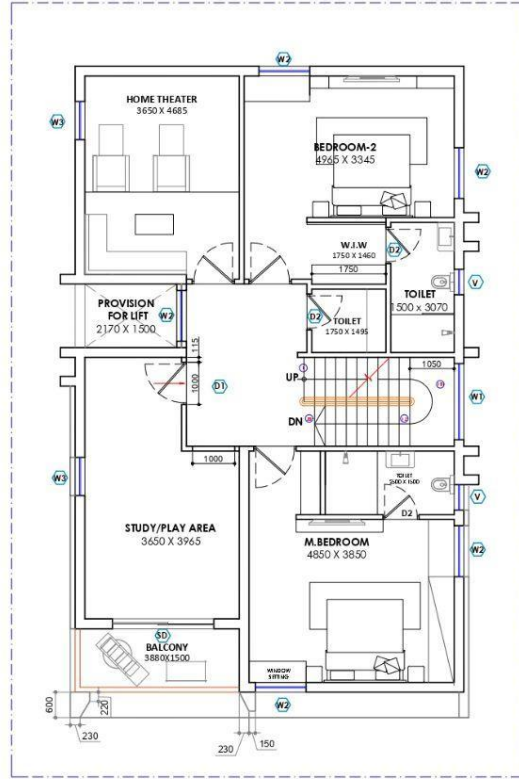
FIRST FLOOR PLAN V-31 (18-03-2023)
