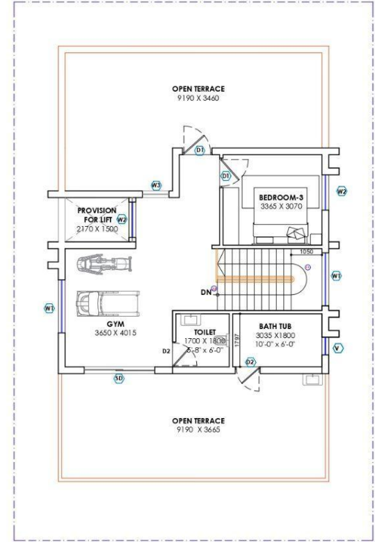
SECOND FLOOR PLAN - OP1 V-31 (18-03-2023)
